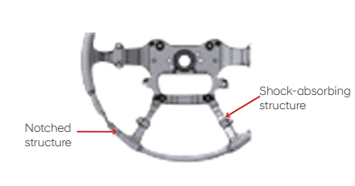
Impact Collapse Wheel The steering wheel automatically collapses in the event of a collision to protect the driver
